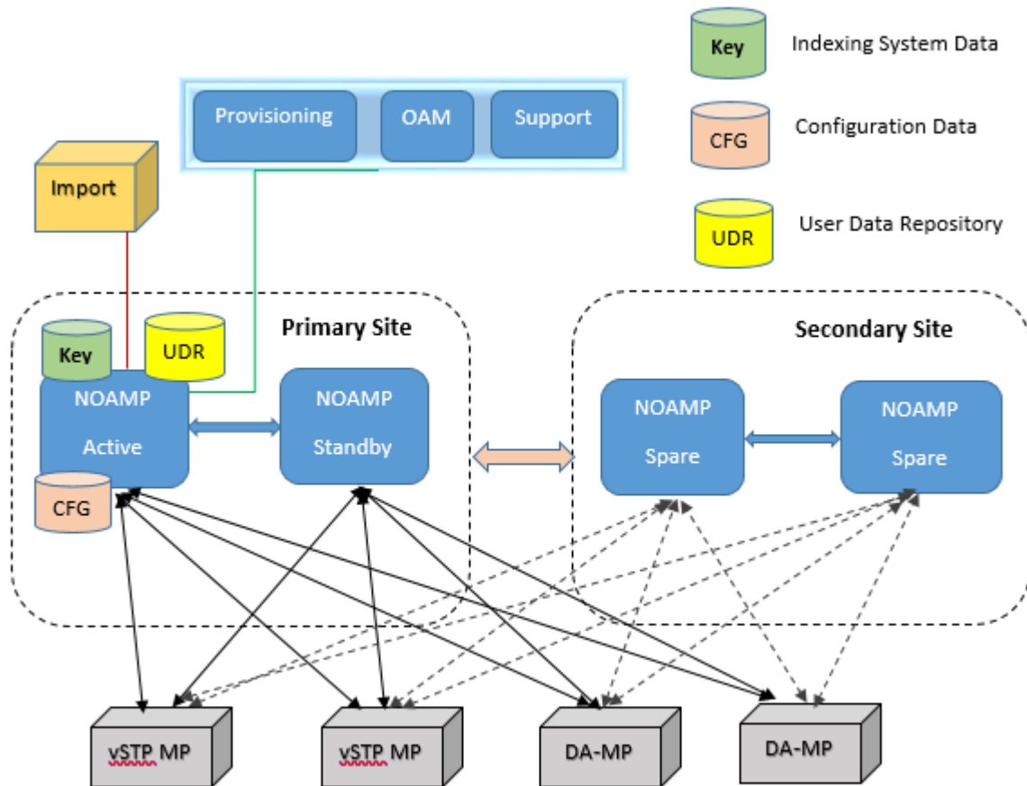
Figure 1: User Data Repository High Level Architecture
